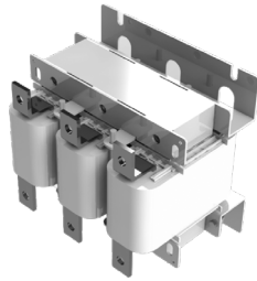
Bus-Bar Type[55~220kW]
