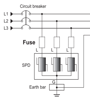
삼상접지(3P3W) (3phase earthed type)
